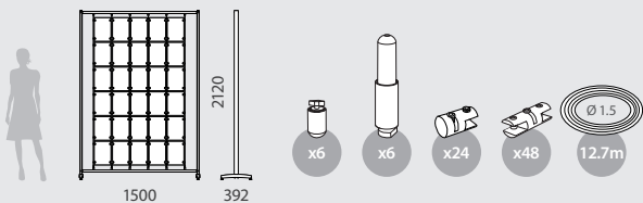
12356 FREE STANDING
